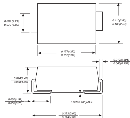
DO-214AC
