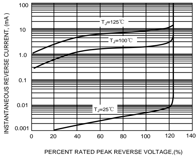
FIG. 5-TYPICAL REVERSE CHARACTERISTICS
