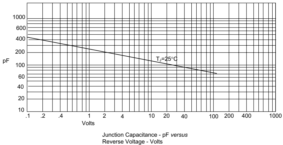
Figure 3 Junction Capacitance
