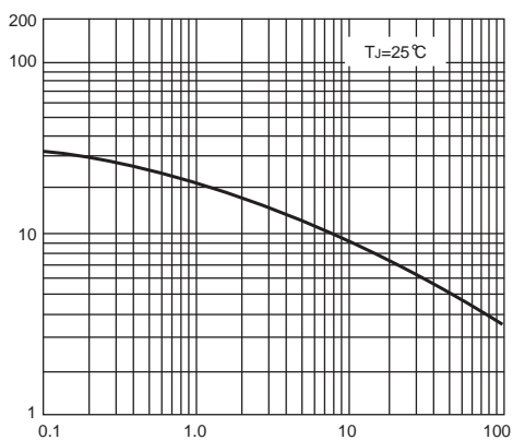
FIG. 5-TYPICAL JUNCTION CAPACITANCE
