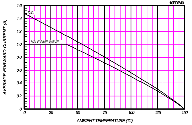
AVERAGE FORWARD CURRENT VS. AMBIENT TEMPERATURE P.C. Board mounted (L=3mm,Print Land=5x5mm,Both Sides)
