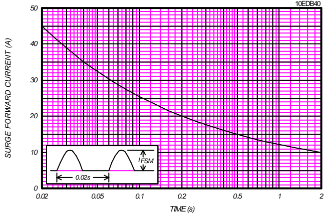
SURGE CURRENT RATINGS f=50Hz,Half Sine Wave,Non-Repetitive,No Load
