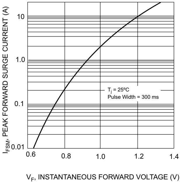
Fig. 1 Peak Forward Surge Current vs Forward Voltage
