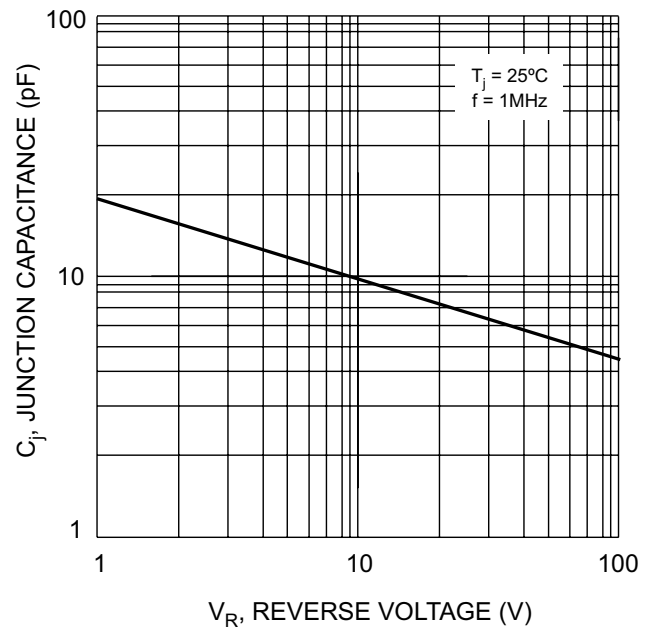
Fig. 4 Junction Capacitance vs Reverse Voltage
