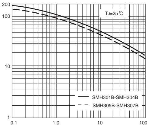
FIG. 5-TYPICAL JUNCTION CAPACITANCE
