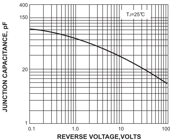
FIG. 5-TYPICAL JUNCTION CAPACITANCE
