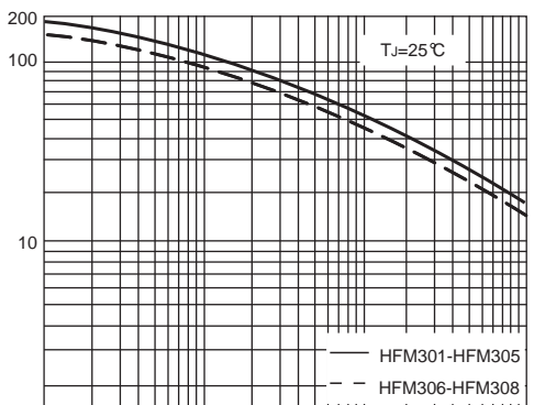
FIG. 5-TYPICAL JUNCTION CAPACITANCE
