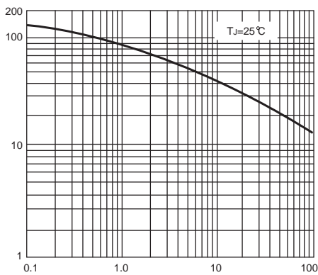
FIG. 5-TYPICAL JUNCTION CAPACITANCE
