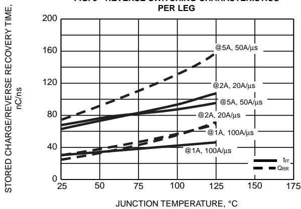
FIG. 5 - REVERSE SWITCHING CHARACTERISTICS PER LEG
